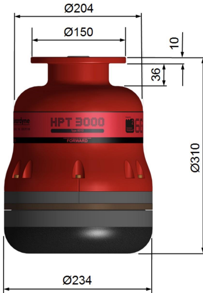
Figure B-7 HPT 3000 Dimensions
