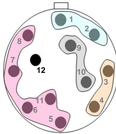
SOLDERING VIEW
