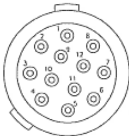
FACE VIEW
